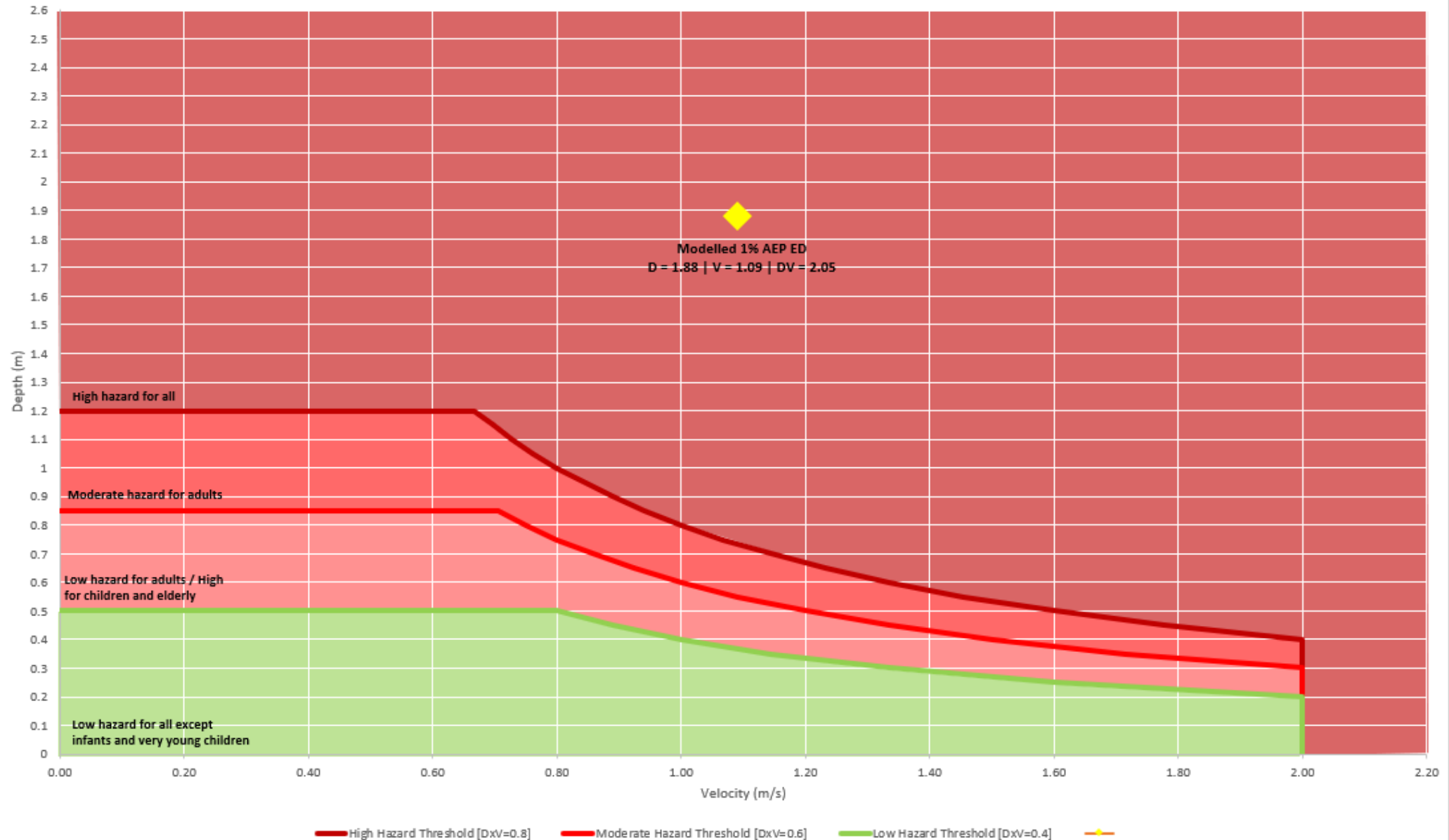
Depth x Velocity Chart 2 - Flood Hazard Thresholds for Person Stability Outside
