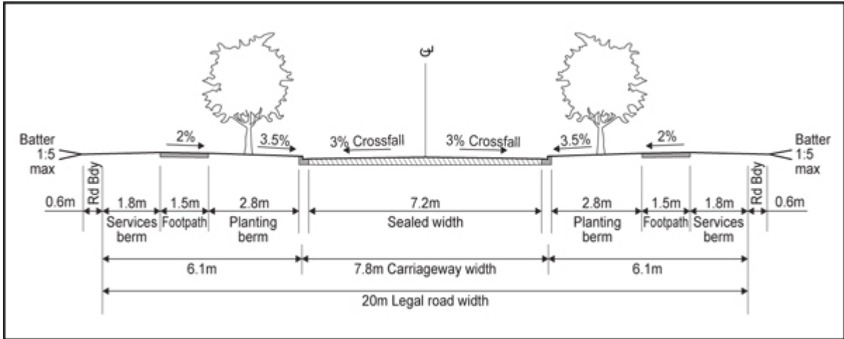
Figure I408.6.7.2 Proposed typical rural interface local road
