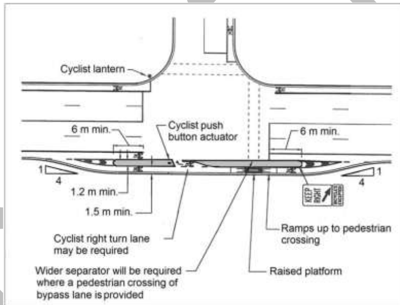
Figure 39: Cyclists bypass at signalised T-intersection (Source Cycling Aspects of Austroads Guides Figures 5.9)
