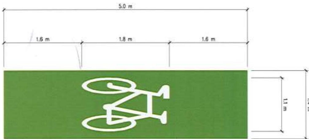
Figure 19: Cycle lane symbol
