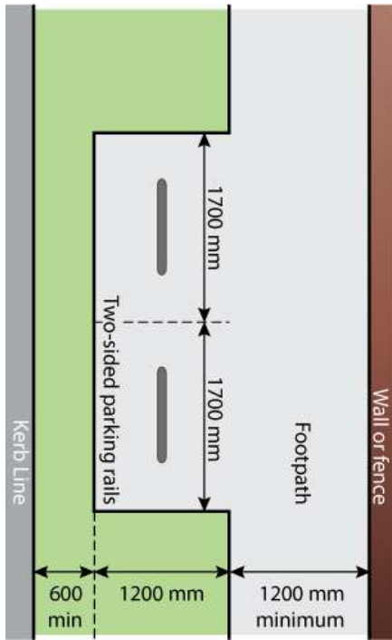
Figure 51: Nose to Tail Parking Both Sides of Rail (Austroad)
