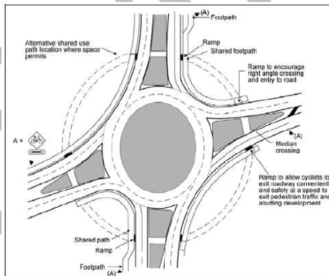
Figure 26: Roundabout treatment for high traffic flows and low cycle traffic flows (from Austroads)
