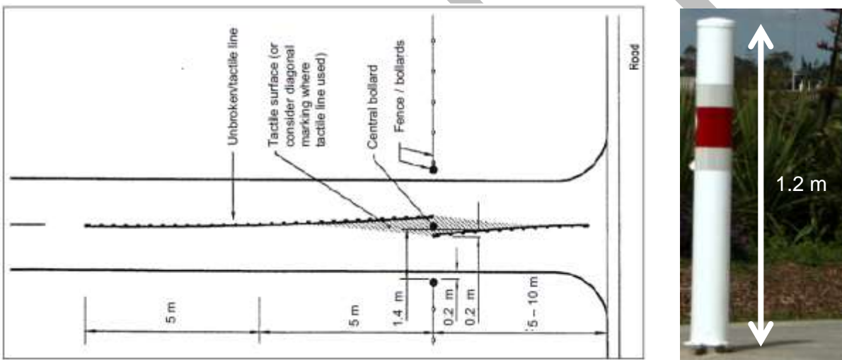
Figure 35: Layout and marking for the use of central bollard (Source: Figure 10.2 Austroads Part 6A 2009)
