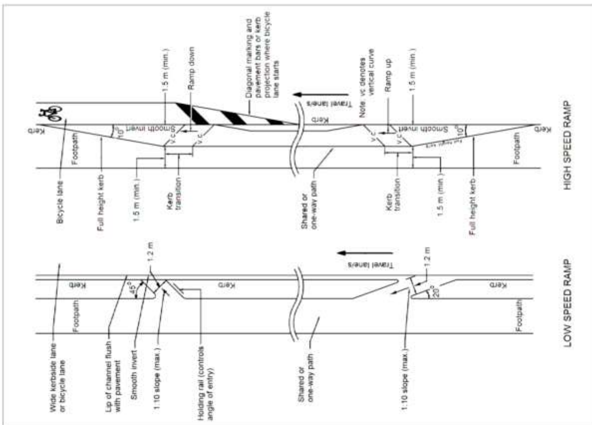
Figure 38: Low and high speed exit and entry ramps (Source: figure 4.10 Cycling aspects of Austroads)
