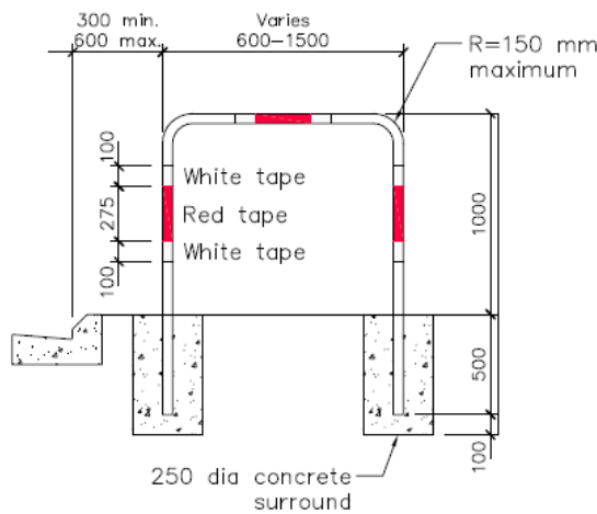
Figure 29: Cyclist holding rail detail
