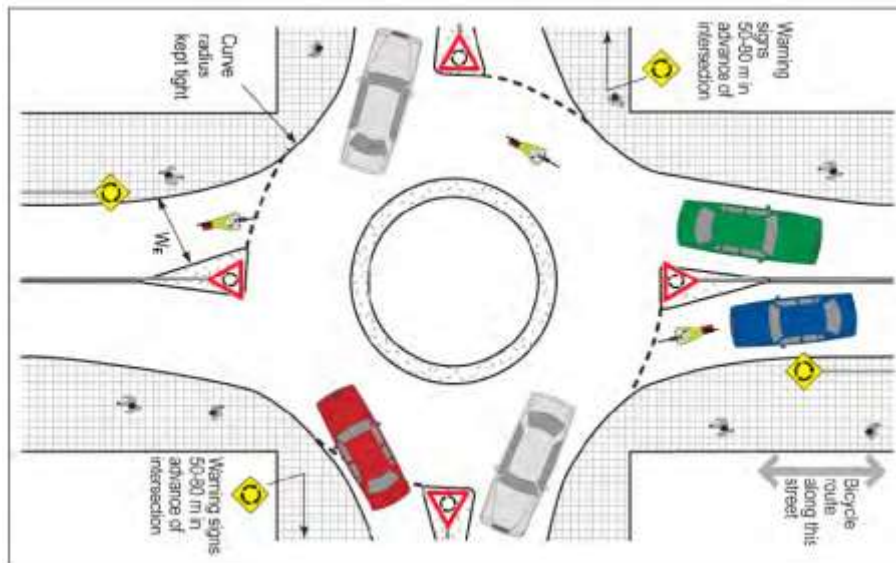
Figure 25: Roundabout treatment for slow speeds and low traffic flows (from Austroads)
