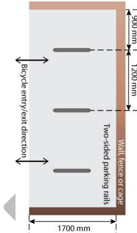
Figure 52: Side by Side Parking 90 degree (Austroad)
