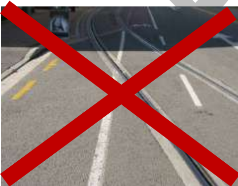
Figure 28: Cycle lane across tram track at oblique angle
