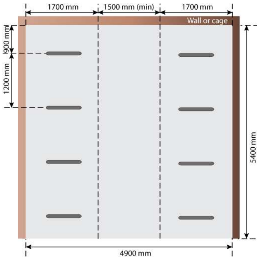
Figure 56: Typical Cycle Parking Layout – 16 Bicycle
