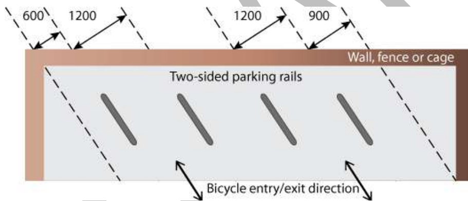
Figure 53: Side by Side Parking - Angle (Austroad)
